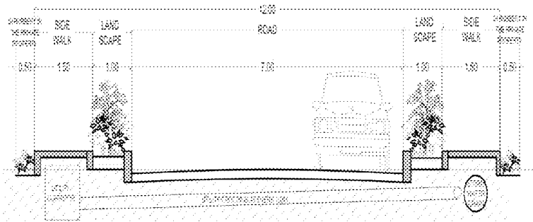
12 M WIDE SECTION
