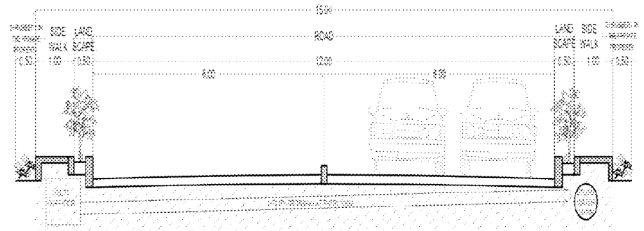
15 M WIDE SECTION
