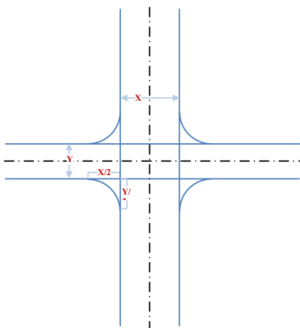
Fig.1: Rounding off at junctions of right-angled intersections
